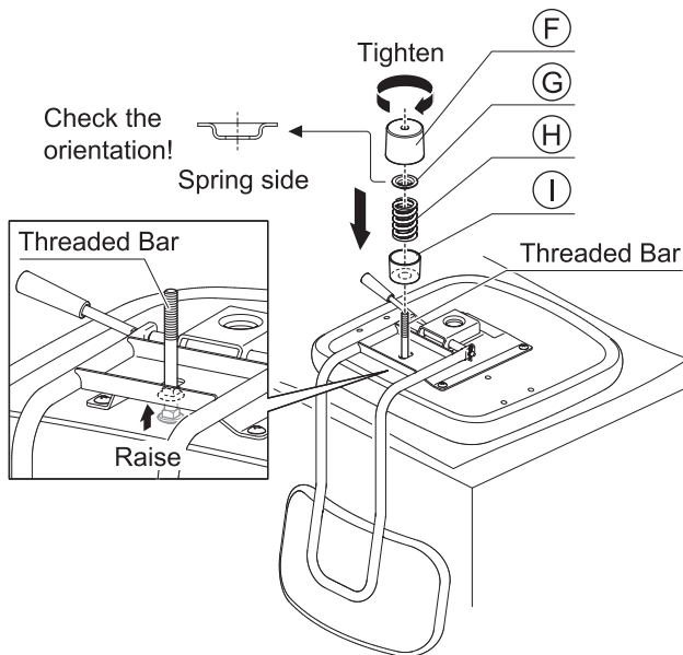
Figure 1 Approximate Handle Tightening Position
