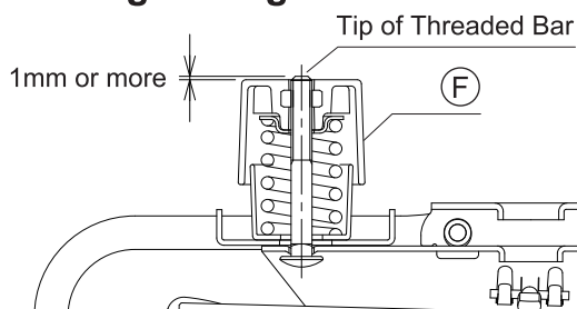
Figure 1 Approximate Handle Tightening Position
